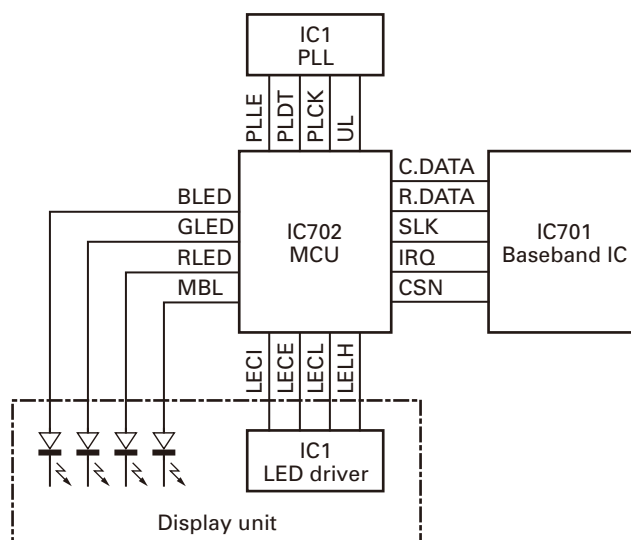
Fig. 10 Control circuit
