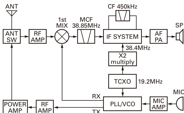
Fig. 1 Frequency configuration
