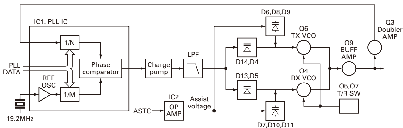
Fig. 8 PLL circuit
