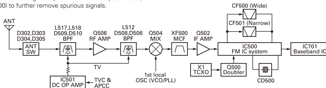
Fig. 2 Receiver System
