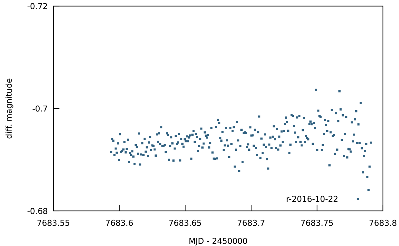
wasp-74
