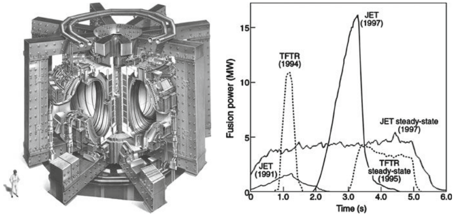
Fig. 1.17 (a) The JET tokamak is 12 m high and has a D-shaped plasma cross-section and a total plasma volume of 80–100 m 3 (Image: EFDA-JET). (b) Fusion power development in the D-T campaigns of JET and TFTR. (Graphic: EFDA/JET. Reprinted with permission from [42]. © 2006, American Nuclear Society)
