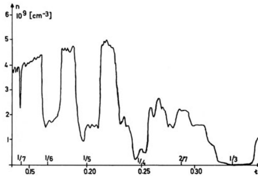
Fig. 3.21 Plasma density in the Wendelstein IIa stellarator for a toroidal magnetic field of 0.6 T and varying rotational transform. The electron density breaks down at rational values \iota/2\pi = 1/3, 1/4, 1/5, \dots (Reprinted with permission from [63]). © IPP/MPG
