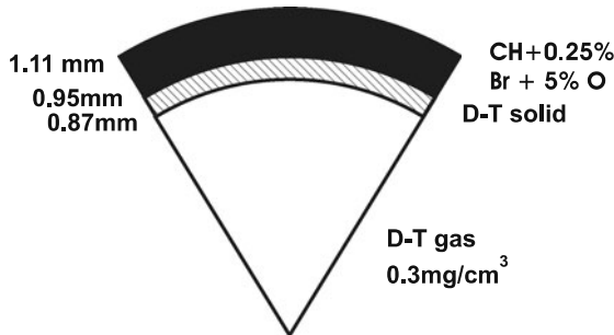
Fig. 4.23 NIF pellet design. A plastic microsphere with the main fuel as a hollow shell of D–T ice. The volume is filled with D–T gas at 30 bar normal pressure to form a hot spot. (Reprinted with permission from [52]. © 2004, American Institute of Physics)
