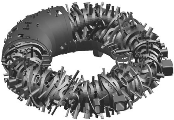
Fig. 1.19 Conceptual view of Wendelstein 7-X, a stellarator experiment with non-planar superconducting field coils. (Reproduced with kind permission. © IPP/MPG)
