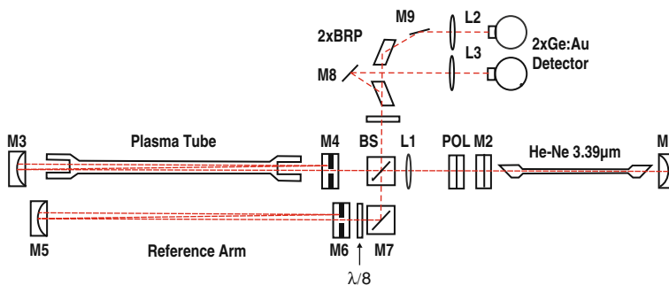
Fig. 6.7 Laser interferometer at \lambda = 3.39\mu\text{m} with folded beams and quadrature detection. The basic concept is a Michelson type interferometer. The \lambda/8 plate generates the circular polarization after two passages. Separation of the two interference signals is achieved with total reflection at the Brewster angle (from [102])
