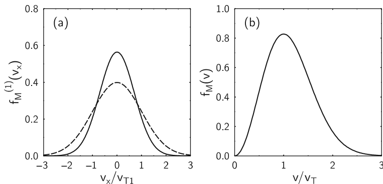
Fig. 4.1 (a) One-dimensional Maxwell distribution f_M^{(1)}(v_x) for two different temperatures. Solid line: T_1 , dashed line: T_2 = 2T_1 . (b) Maxwell distribution f_M(v) of particle speeds
