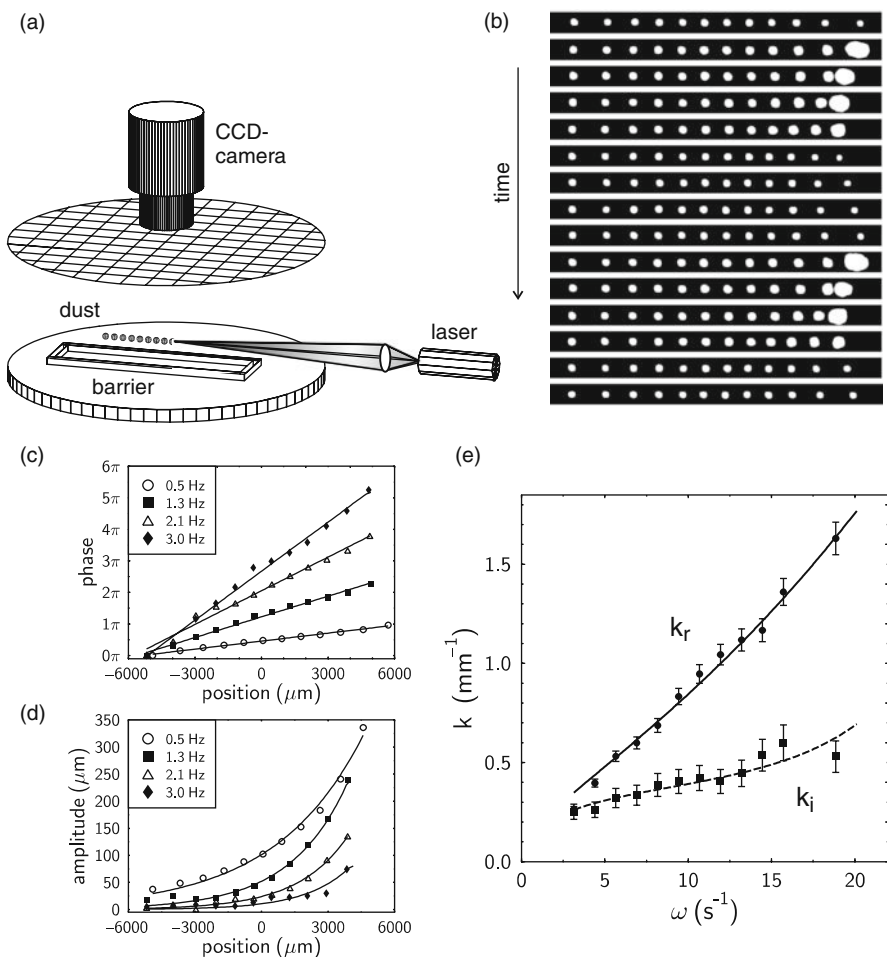
Fig. 10.40 Laser-excited phonon on linear chain. (a) Experimental set-up. (b) Response of particles on chopped laser radiation pressure (inverted image). (c) Phase, (d) amplitude response of the linear chain. (e) Best fit to dispersion and damping by varying \kappa (from [326])
