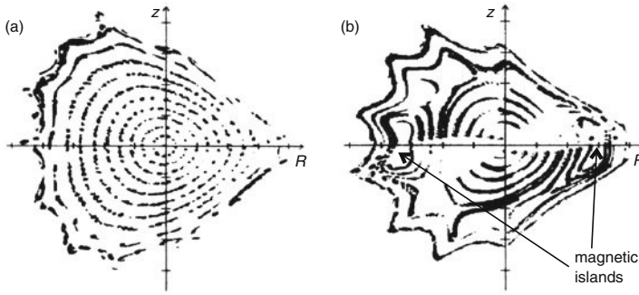
Fig. 3.20 Visualization of the rotational transform by an electron beam and a small movable phosphor screen in the Wendelstein 7-AS stellarator. (a) Nested magnetic surfaces for \iota/2\pi = 0.47 . (b) Magnetic islands form at \iota/2\pi = 1/2 . (Reprinted with permission from [64]. © 1993, IAEA.)
