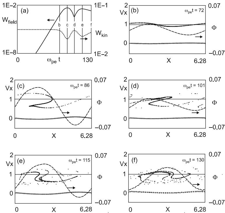
Fig. 9.22 Particle-in-cell simulation of the beam-plasma instability for \alpha_b = 0.01 (a) Semi-log plot of the electric field energy (full line) and beam kinetic energy (dashed line). (b–f) x-v_x phase space showing plasma electrons at v \approx 0 and beam electrons at v \approx 1 . For comparison, the wave potential (long-dashed line) is superimposed. The selected examples correspond to the times marked by vertical lines in panel (a)
