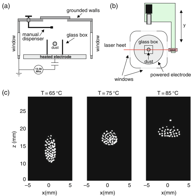
Fig. 10.33 (a) Experimental arrangement for generating Yukawa balls by thermophoretic levitation. (b) Camera and laser for scanning video microscopy. (c) Yukawa balls for different temperature gradients (from [36, 242])
