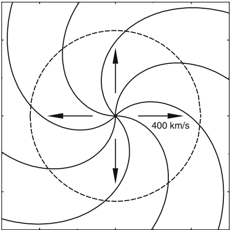
Fig. 1.5 The sun rotation shapes beams of solar wind, which emerge from distinct spots, into an Archimedian spiral. The motion of the solar wind is radially outward, but the magnetic field is trapped in the spiral arms. The Earth orbit is indicated by the dashed circle
