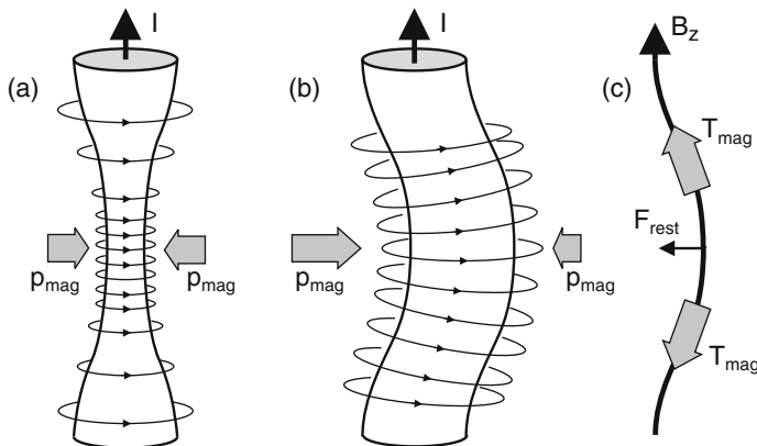
Fig. 8.13 (a) Sausage instability, (b) kink instability of a pinch plasma. The magnetic pressure increases when the cross-section shrinks or becomes asymmetric when the plasma column is curved. (c) The magnetic tension of a superimposed longitudinal magnetic field counteracts the instability
