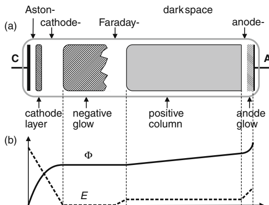
Fig. 11.2 Anatomy of a glow discharge in a long cylindrical tube with plane cathode (C) and anode (A). (a) Various dark spaces and luminous regions are indicated. (b) Sketch of the electric potential \Phi and axial electric field E in the normal glow discharge
